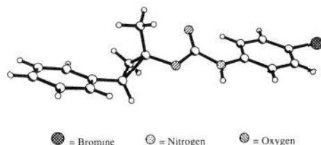
Figure 2. Molecular structure and absolute configuration of the ( p -bromophenyl)urethane of chiral cis -1-methyl-2-phenylcyclopropanol ( 4 ), prepared as shown in eq 3) as determined by X-ray crystallography.
