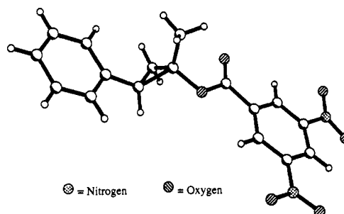
Figure 1. Molecular structure of the 3,5-dinitrobenzoate of cis -1-methyl-2-phenylcyclopropanol as determined by X-ray crystallographic analysis.
